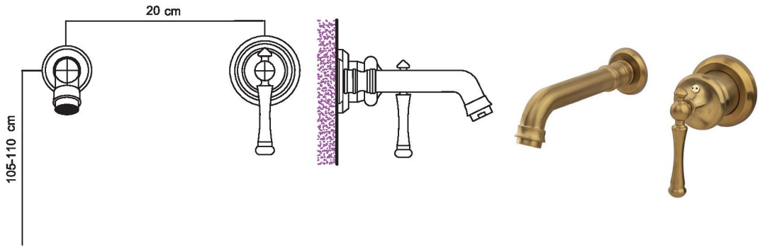
BASIN MIXER
