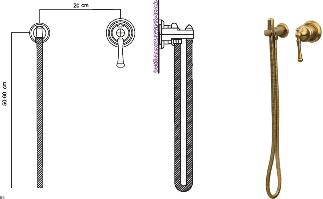
SHOWER MIXER
