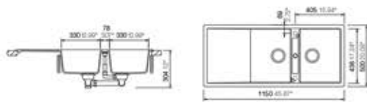
Technical Drawings
