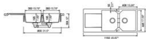
Technical Drawings
