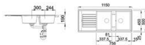
Technical Drawings
