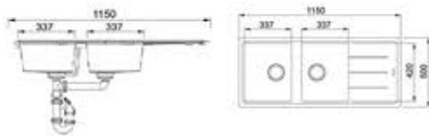
Technical Drawings
